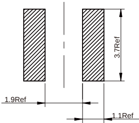
Land Pattern: [mm]
